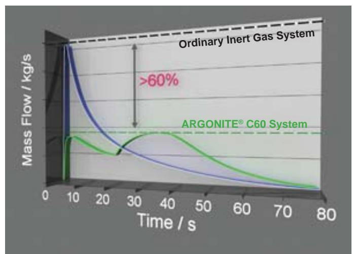
New ARGONITE® C60 Controlled Flow valve
